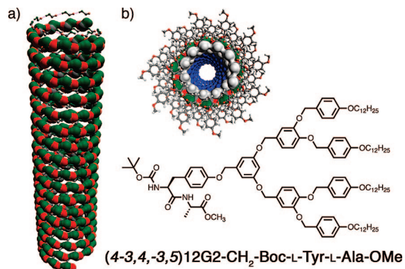
SCHEME 4. (a) The Helical Hydrogen Bonded Supramolecular Polymer Backbone of (4-3,4-3,5)12G2-CH 2 -Boc-L-Tyr-L-Ala-OMe (N=H, Green; O, Red) and (b) Top View of the Supramolecular Pore Lined by the Boc Groups (Blue) a
