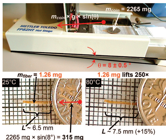
FIGURE 8. Experimental setup that demonstrates the macroscopic scale expansion and contraction of the oriented fiber by the lifting of a dime on the inclined plane of a Mettler hot stage (top). Expanded images collected by a digital camera at 25 °C (bottom left side) and at 80 °C (bottom right side) of the oriented fiber generated from poly[(3,4-3,5)16G2-4EBn] during lifting of 250-times its weight via thermally fueled unwinding of its helix at the \Phi_h^{\text{lo}} -to- \Phi_h transition. Reproduced with permission from ref 53. Copyright 2008 American Chemical Society.
